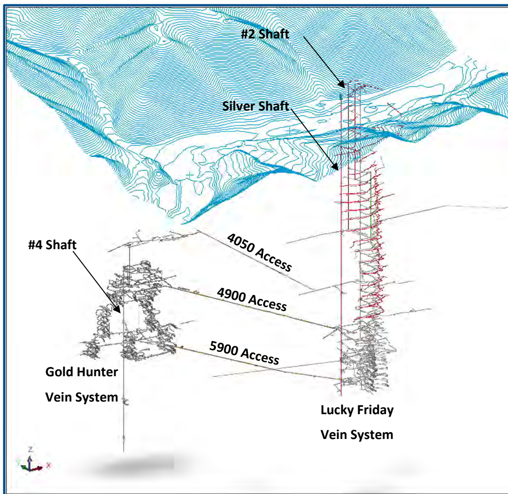
Figure 13-1: Isometric View of As-built Lucky Friday Workings
