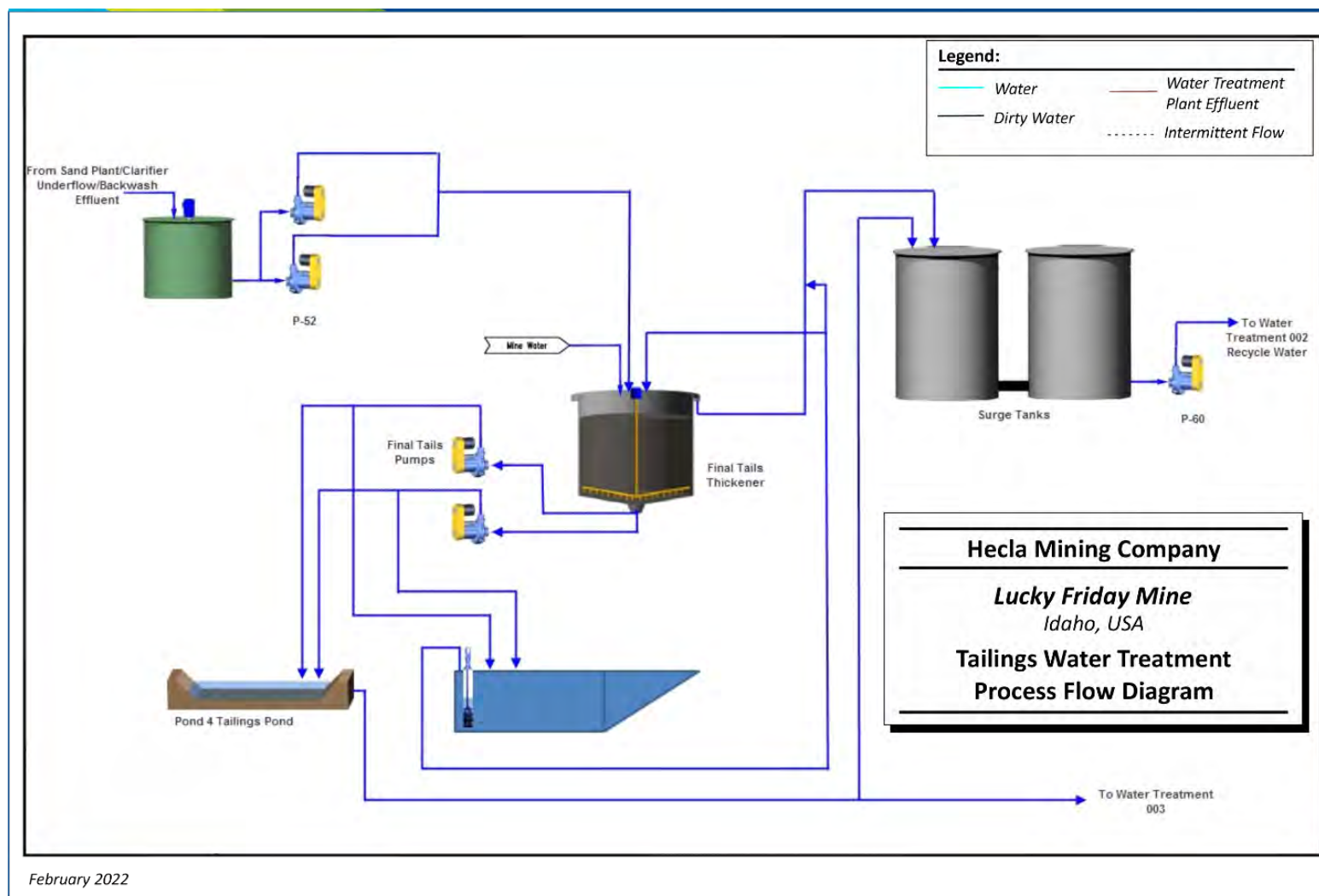
Figure 14-7: Tailings Water Treatment Process Flow Diagram
