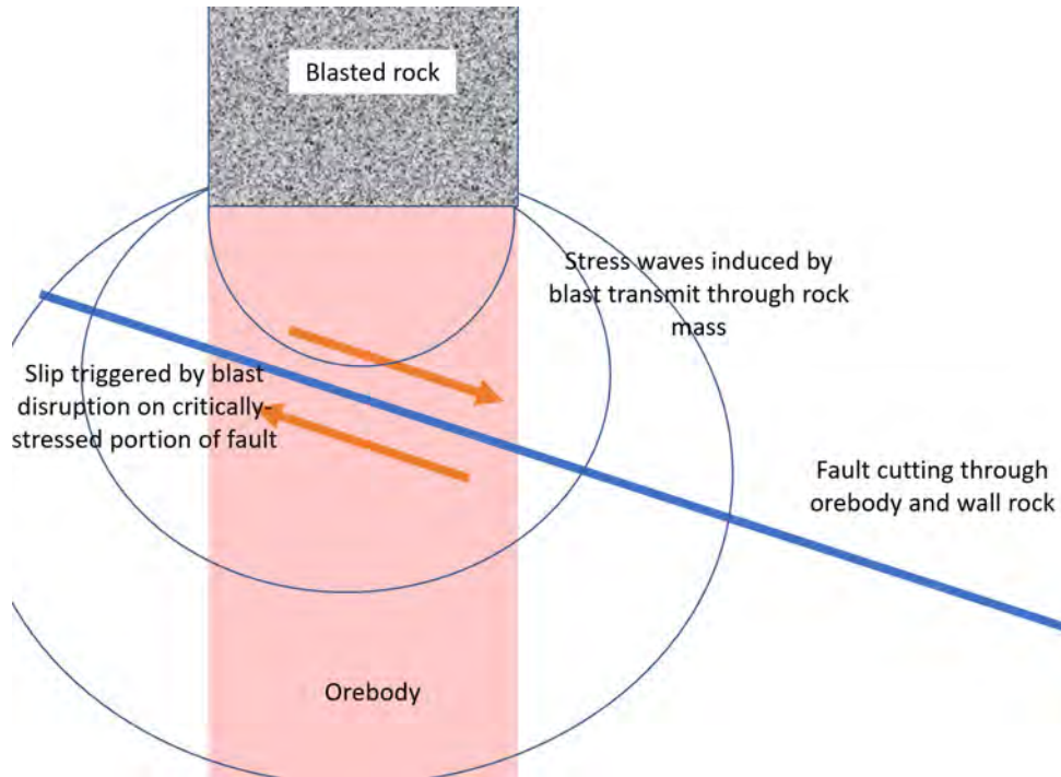
Figure 13-4: Conceptual Fault-Slip in UCB Cross Section
