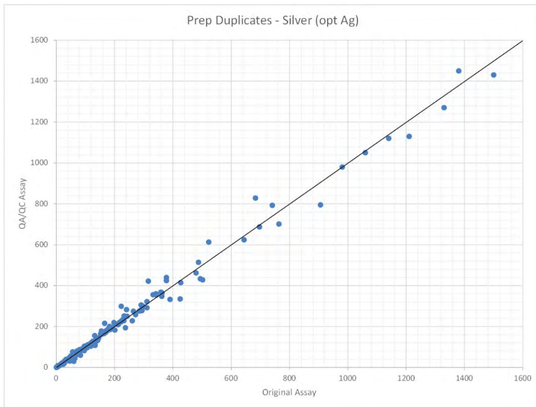
Figure 8-1: Prep Duplicates – Silver
