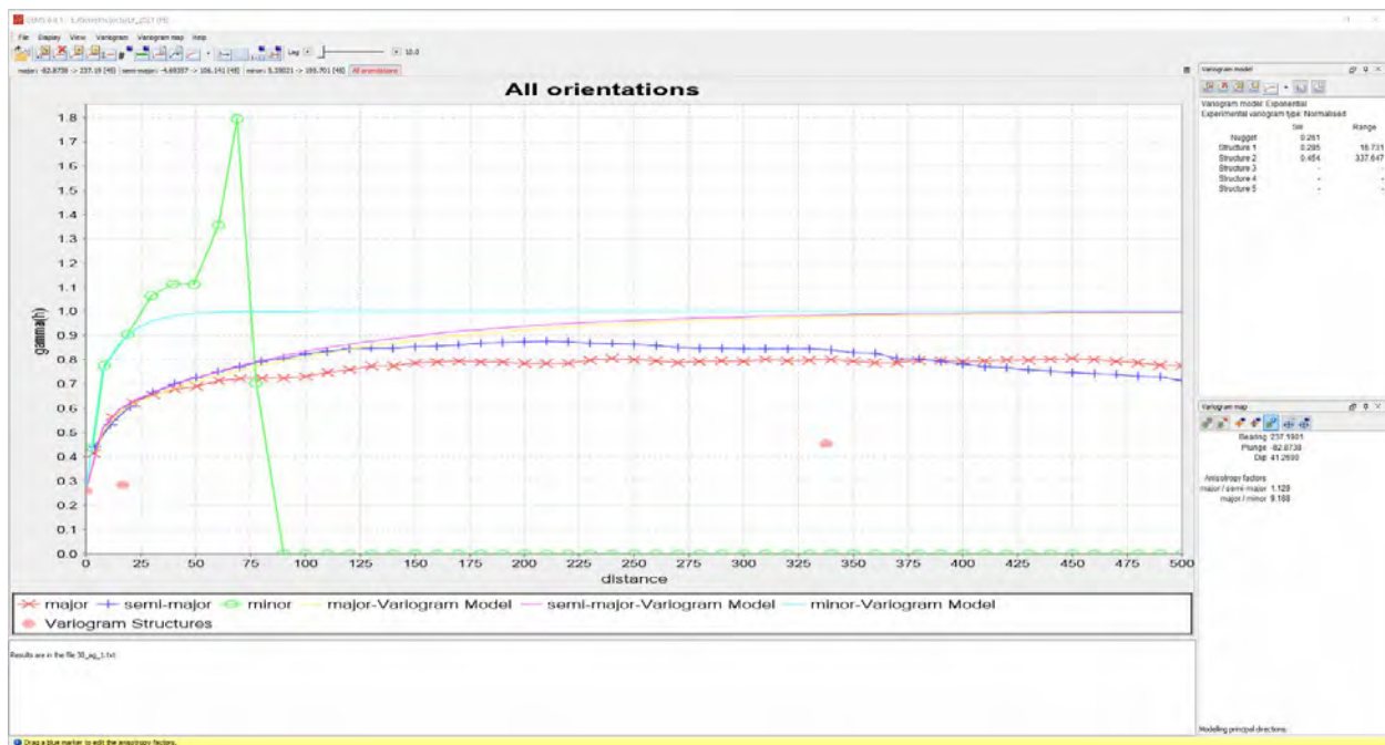
Figure A2: Variogram Model For Iron – 30 Vein
