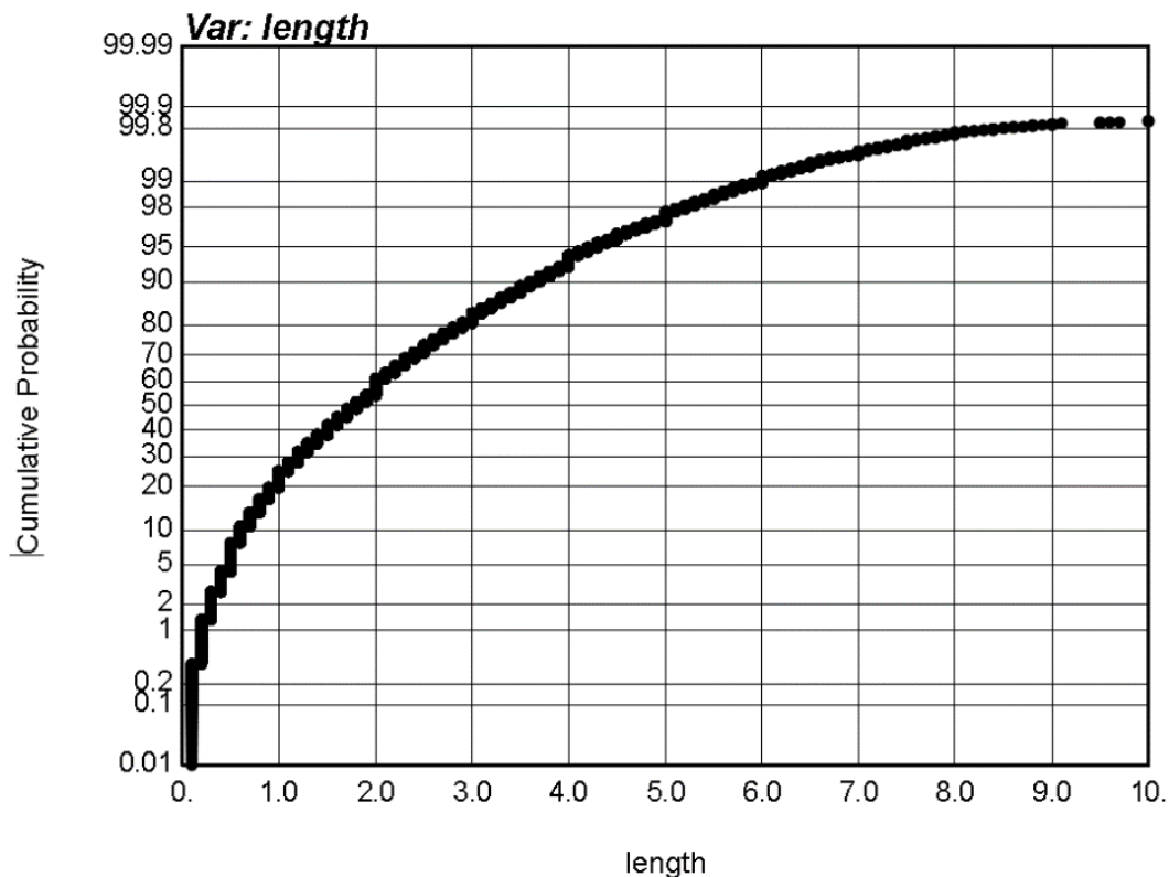
Figure 11-3: Probability Plot of Sample Lengths
