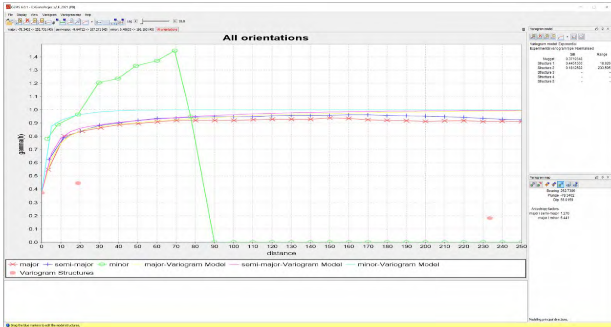
Figure A3: Variogram Model For Lead – 30 Vein
