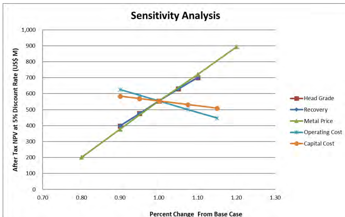
Figure 19-1: After-tax NPV at 5% Sensitivity Analysis
