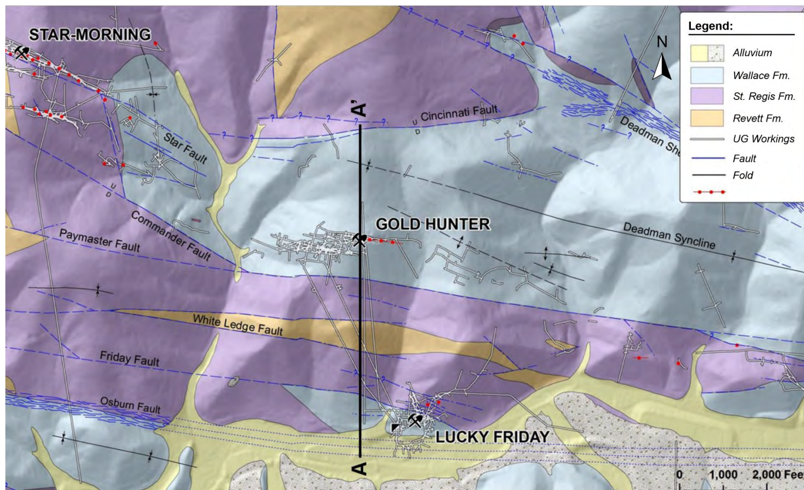
Figure 6-5: Property Geology
