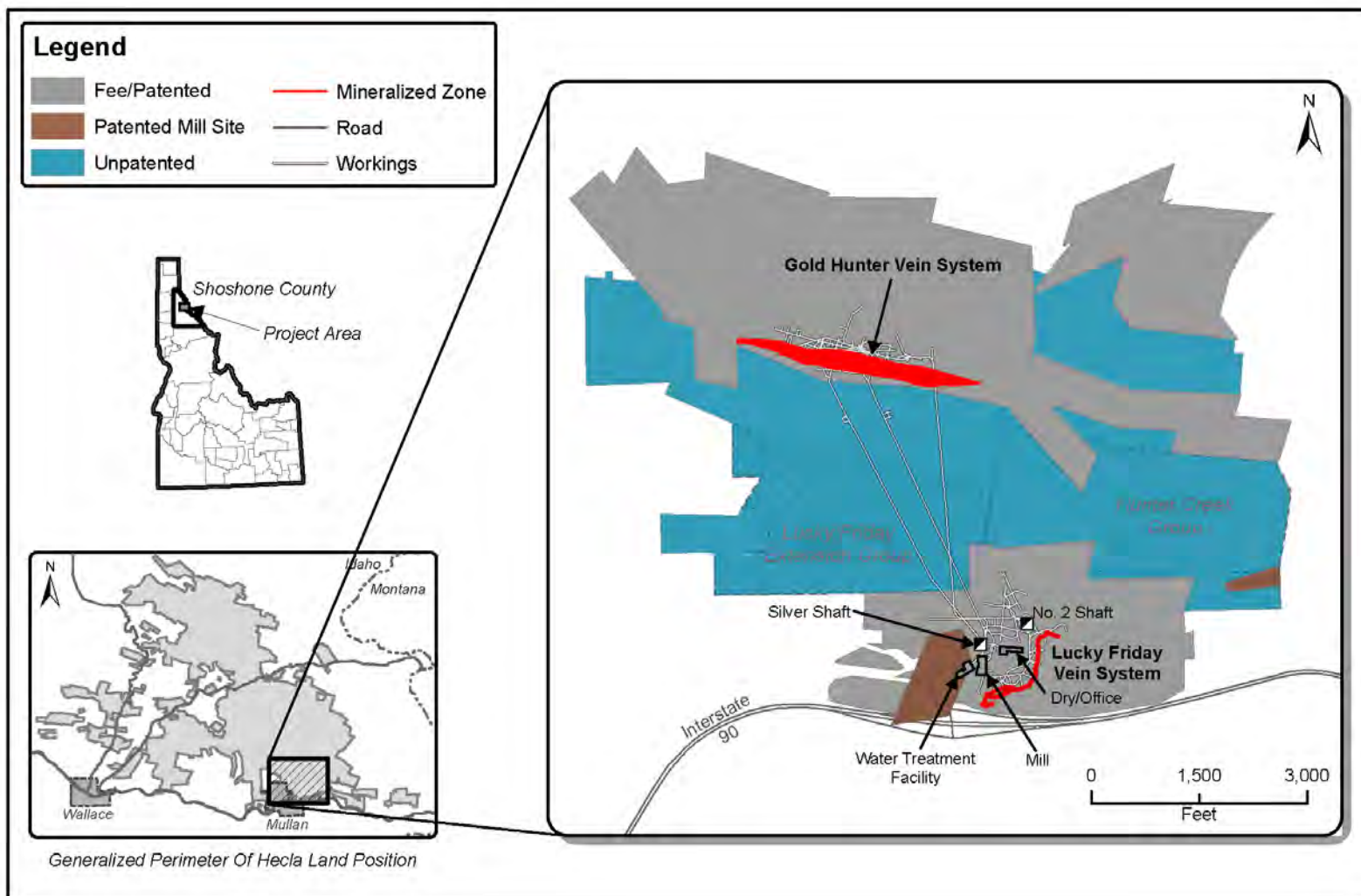
Figure 3-2: Lucky Friday Complex Claim Map
