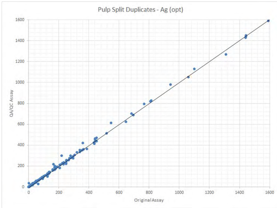
Figure 8-2: Pulp Split Duplicates – Silver
