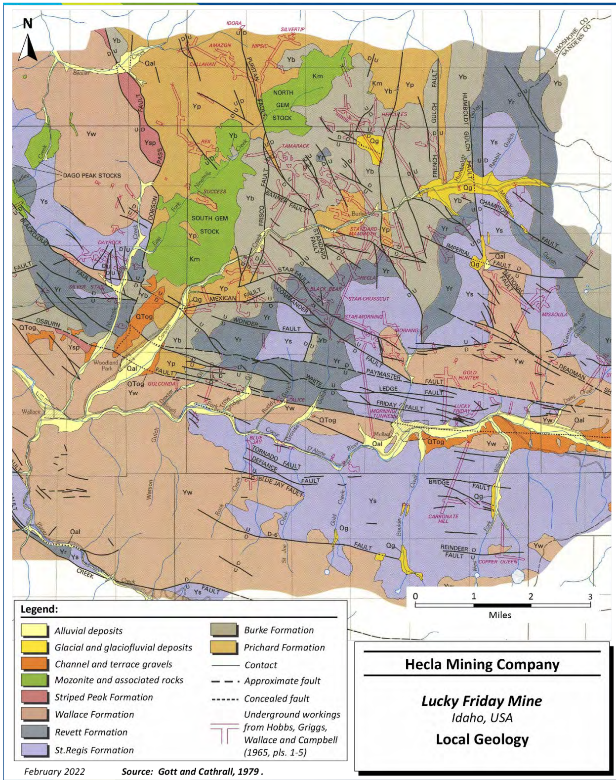
Figure 6-3: Local Geology
