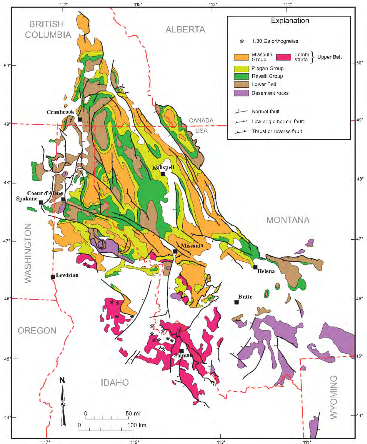
Figure 6-1: Regional Geology
