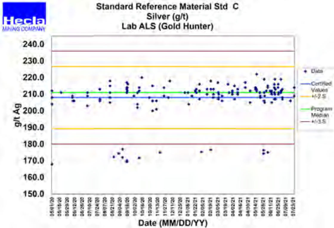
Figure 8-3: Example Control Chart for Silver – Standard C (ALS)
