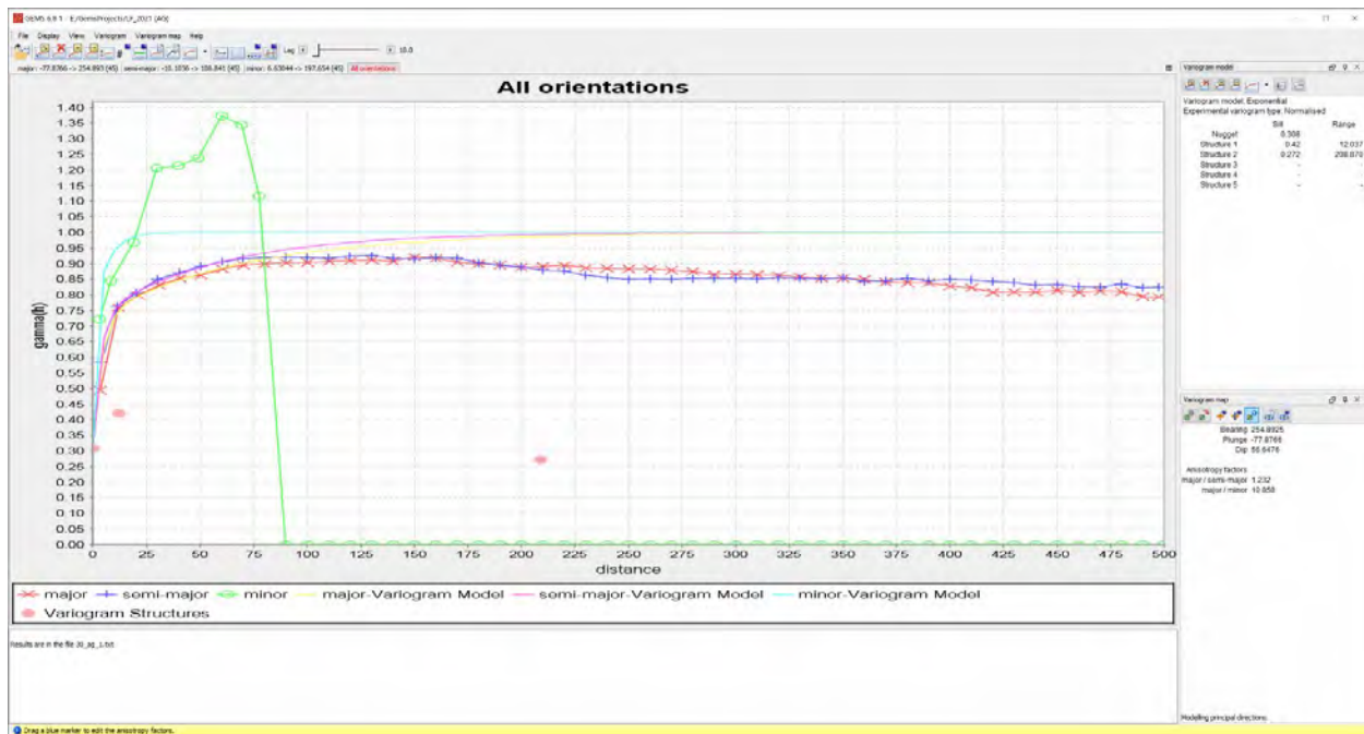
Figure A1: Variogram Model For Silver – 30 Vein
