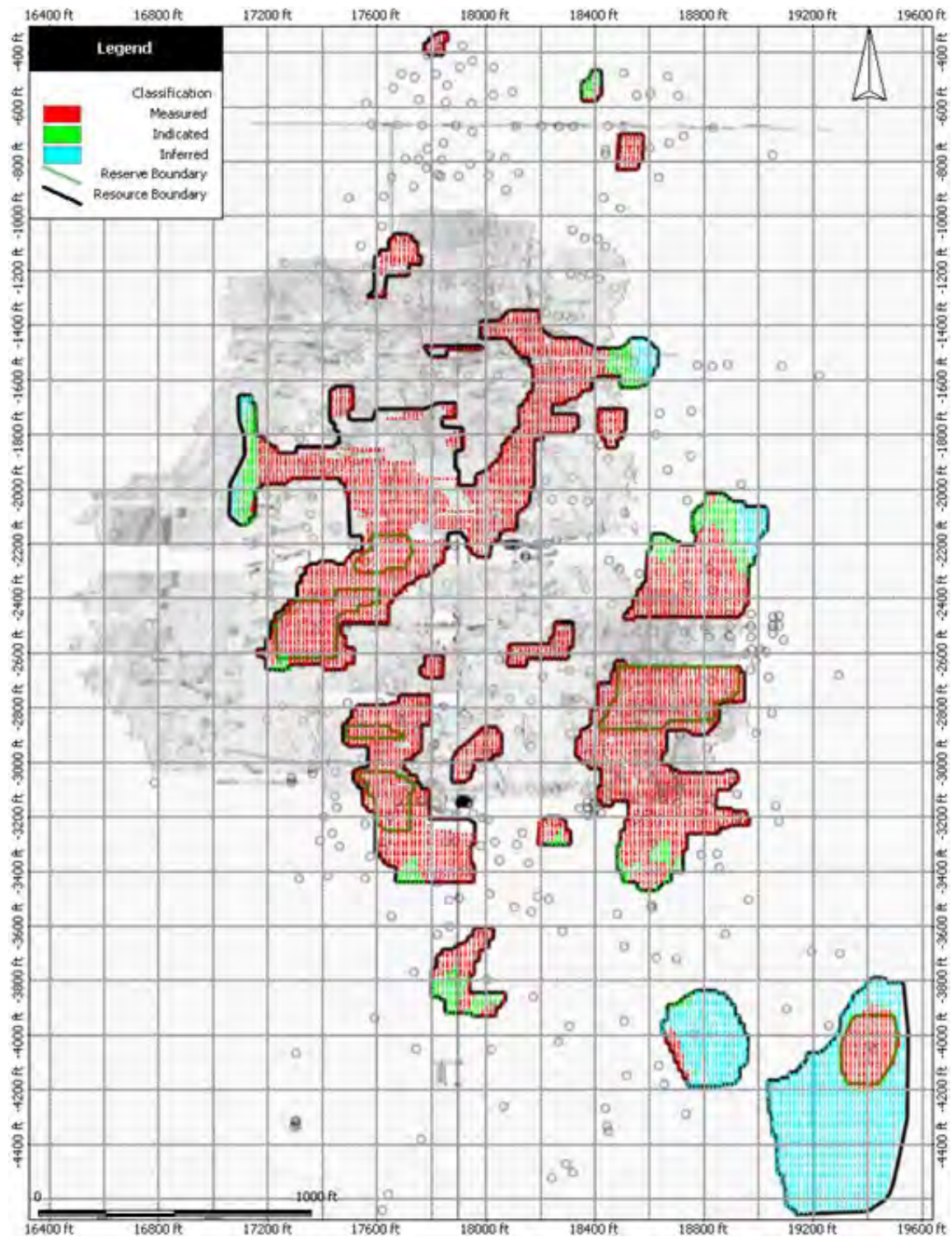
Figure 11-5: 90 Vein Classification
