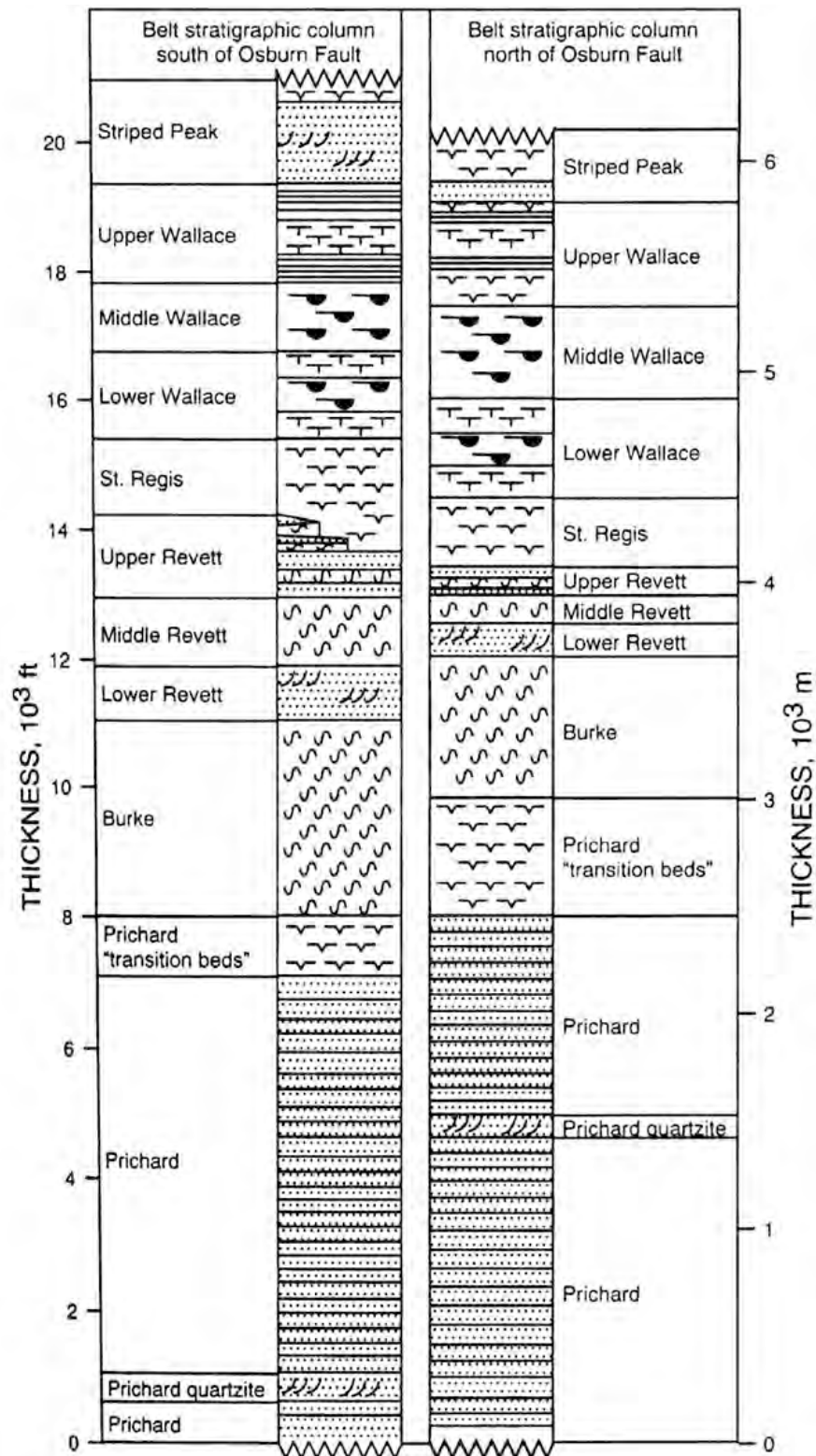
Figure 6-4: Stratigraphic Column
