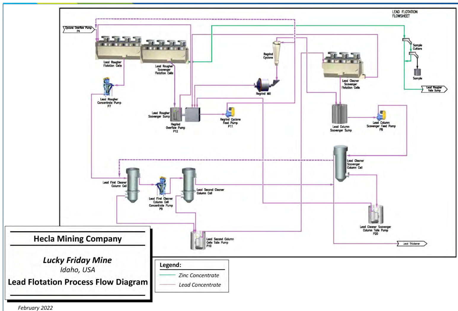
Figure 14-3: Lead Flotation Process Flow Diagram
