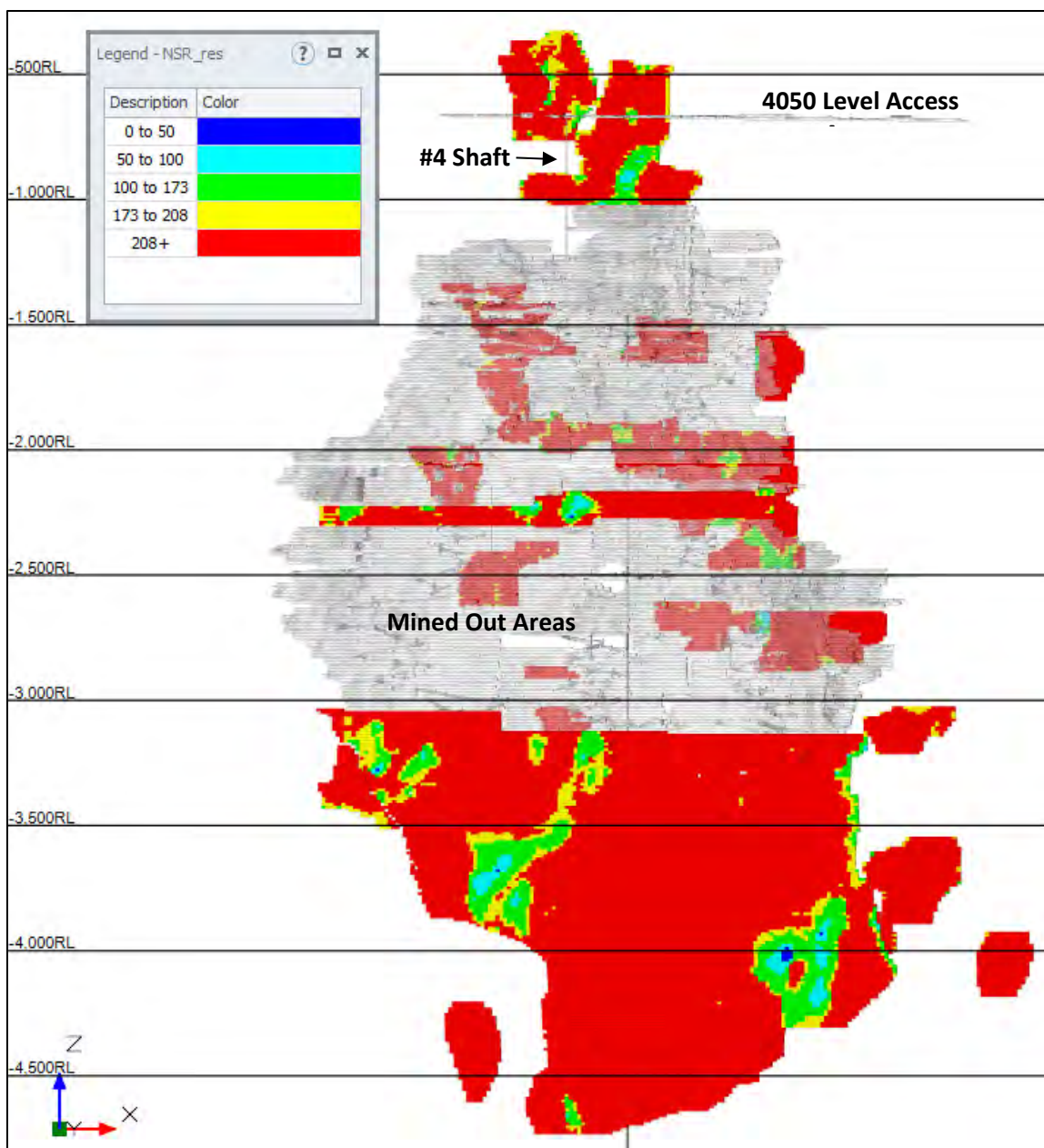
Figure 13-9: Longitudinal Section – 2D View
