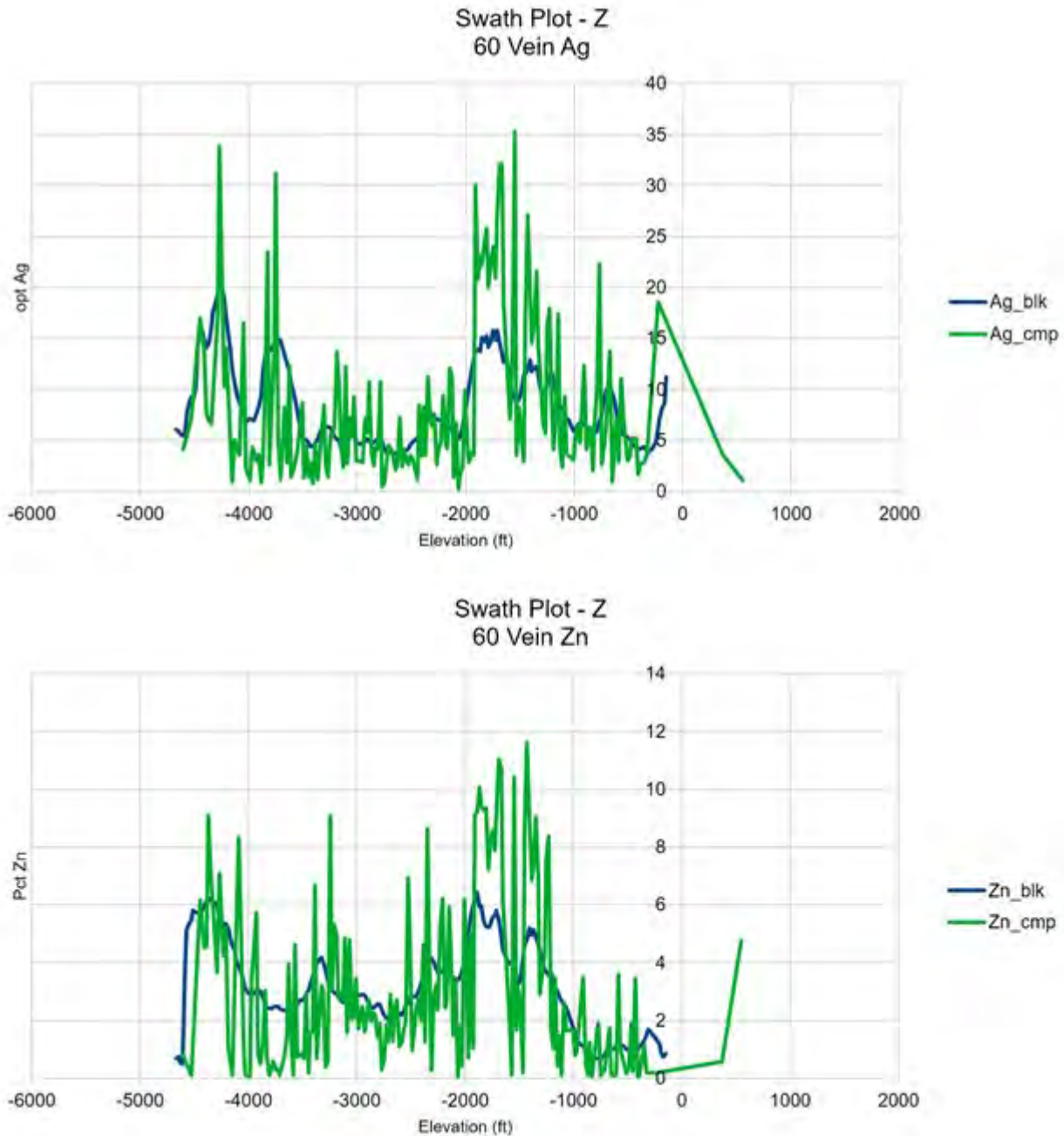
Figure 11-7: Drift Analyses – 60 Vein
