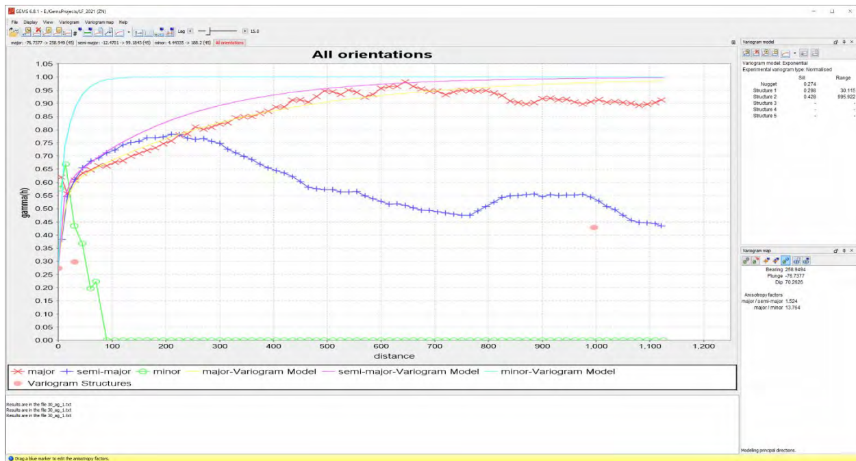
Figure A4: Variogram Model For Zinc – 30 Vein
