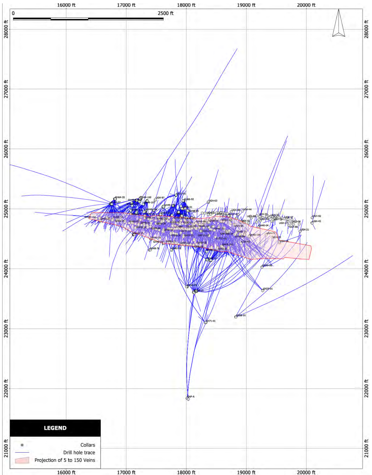
Figure 7-1: Gold Hunter Diamond Drill Plan
