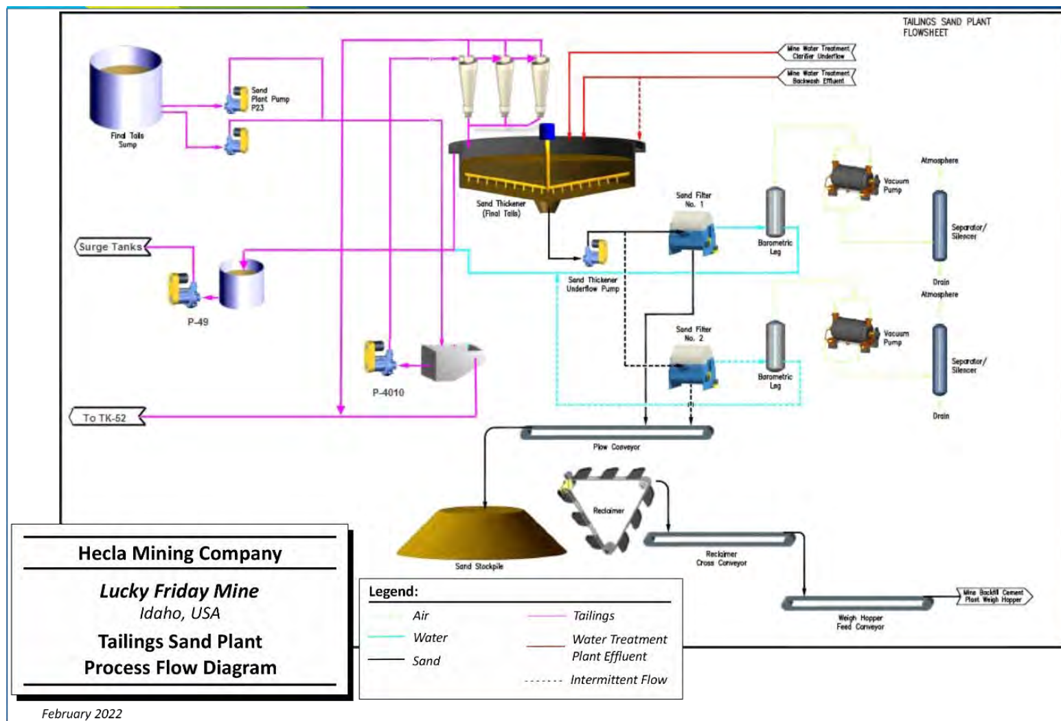
Figure 14-6: Tailings Sand Plant Process Flow Diagram
