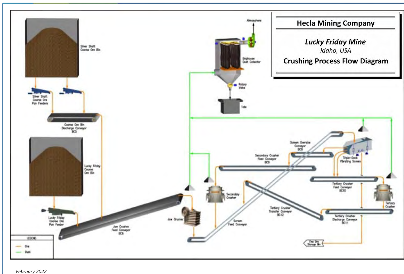
Figure 14-1: Crushing Process Flow Diagram
