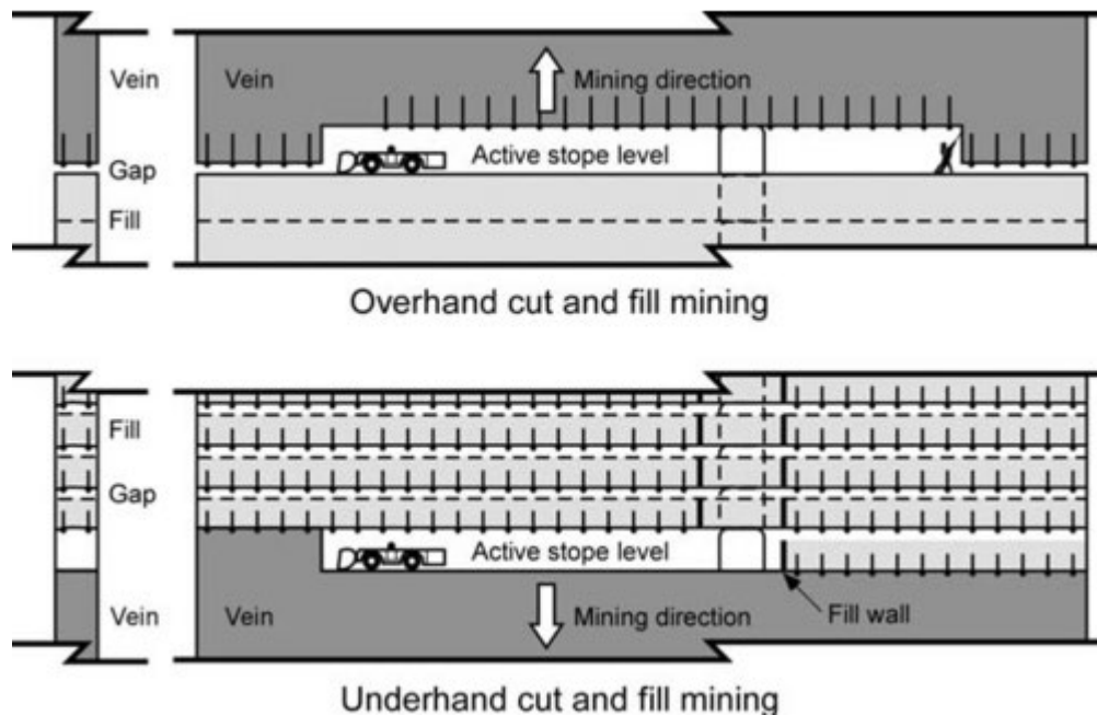
Figure 13-2: Mechanized Overhand and Underhand Stopping
