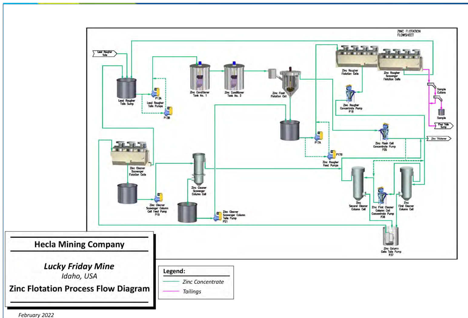
Figure 14-4: Zinc Flotation Process Flow Diagram
