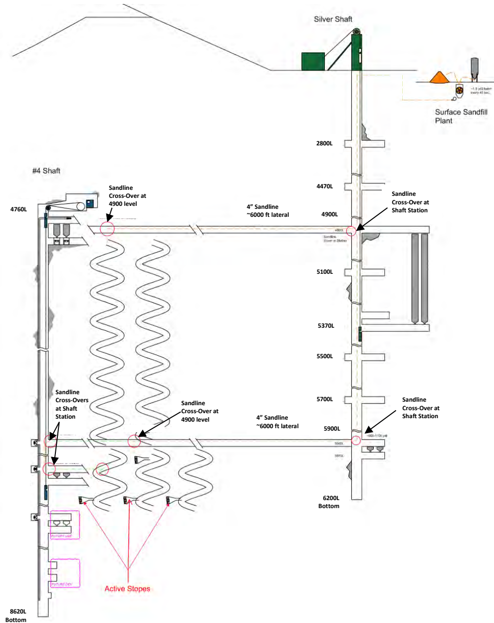
Figure 13-5: Backfill Schematic
