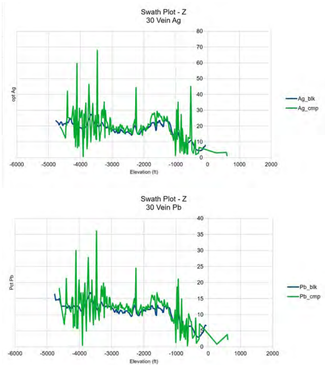
Figure 11-6: Drift Analyses – 30 Vein
