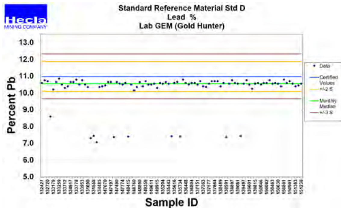
Figure 8-5: Example Control Chart For Lead – Standard D (Gem)
