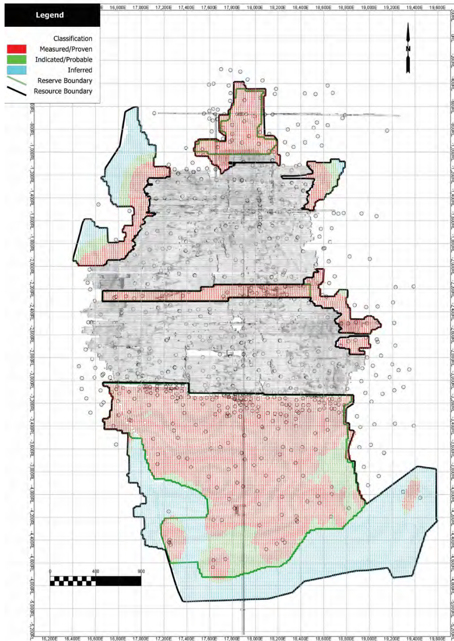
Figure 11-10: Longitudinal Projection – 30 Vein
