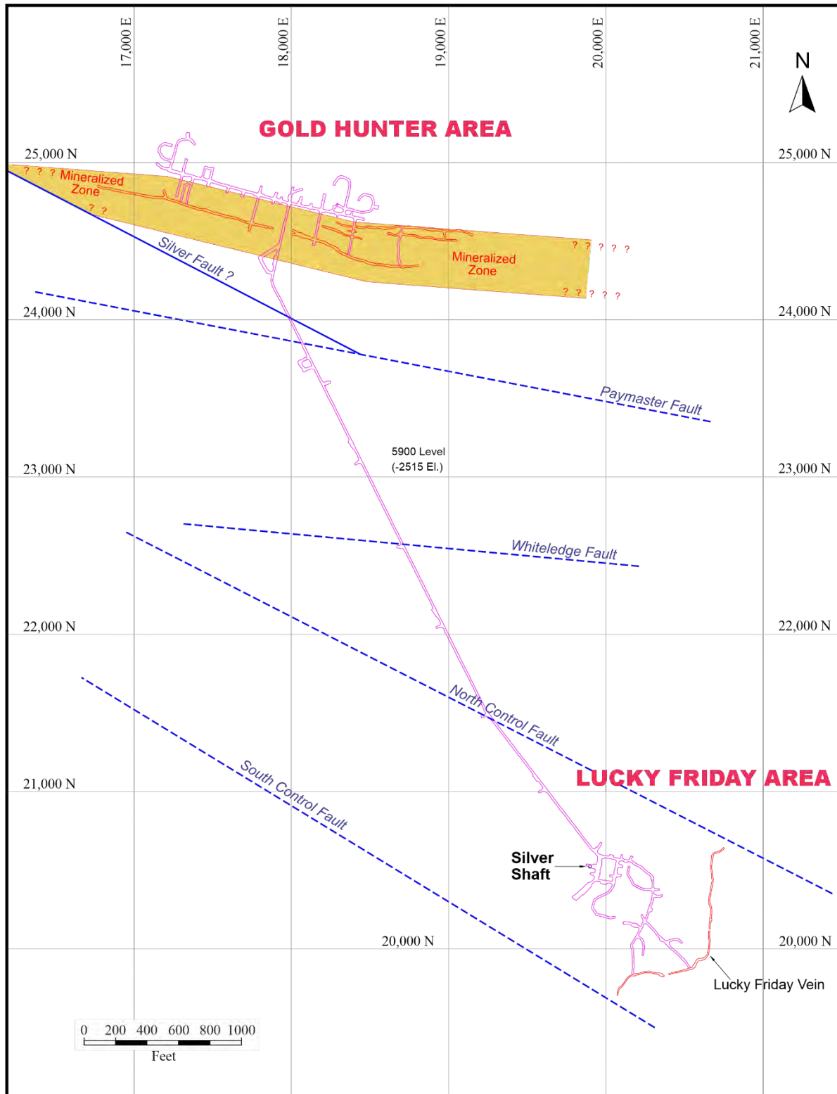
Figure 6-6: Geological Plan 5900 Level
