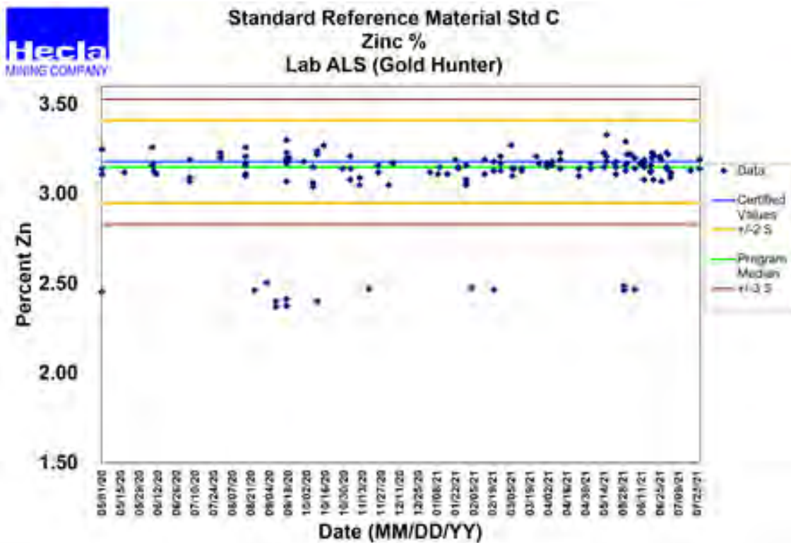
Figure 8-4: Example Control Chart for Zinc – Standard C (ALS)
