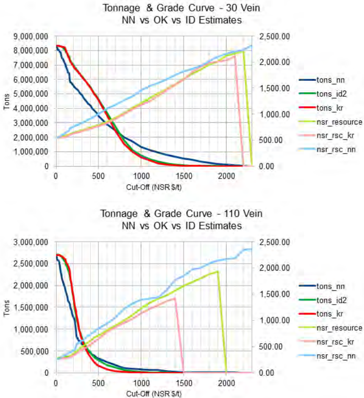
Figure 11-8: Tonnage and Grade Curves
