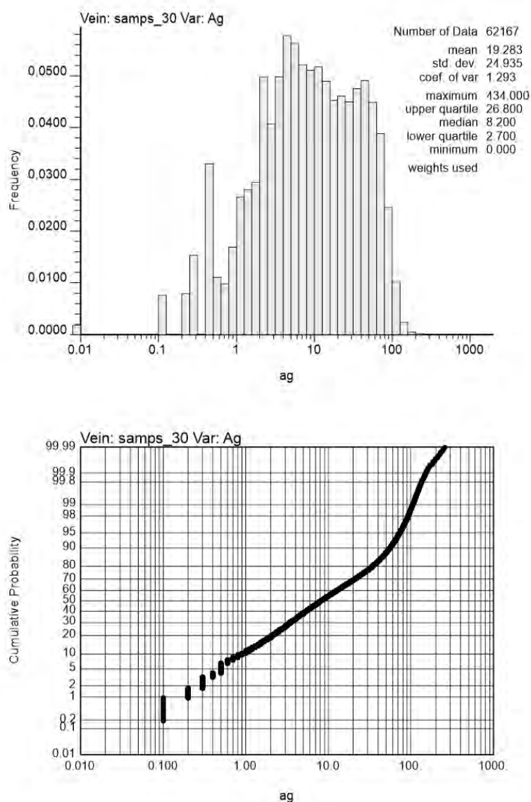
Figure 11-2: Log Histogram and Probability Plot For Silver – 30 Vein
