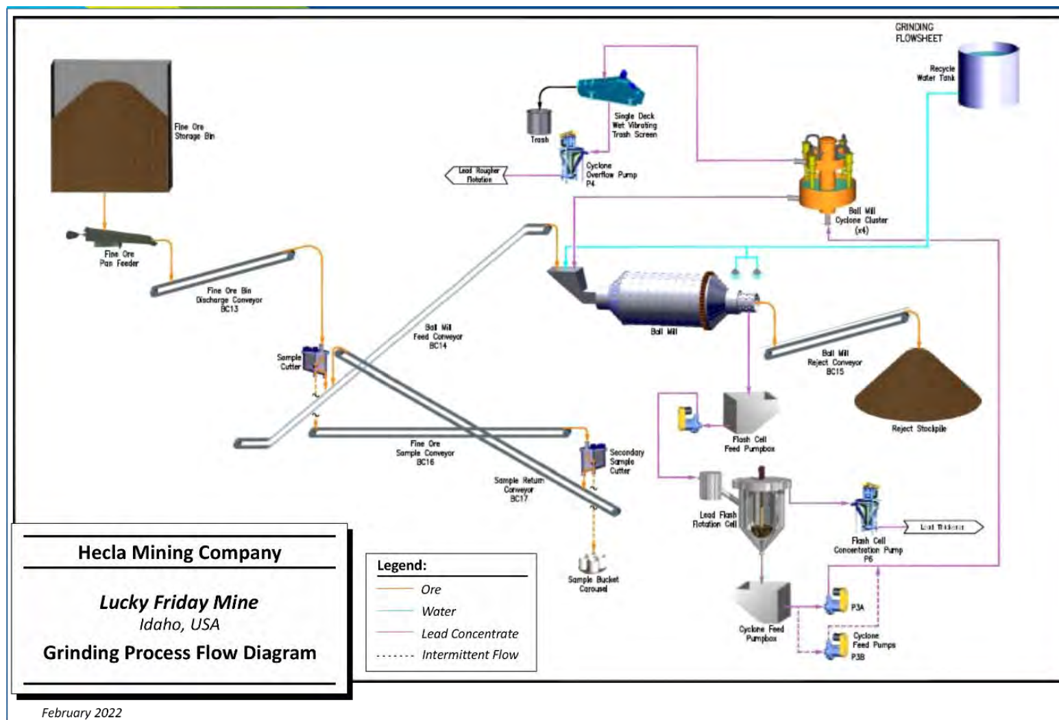
Figure 14-2: Grinding Process Flow Diagram
