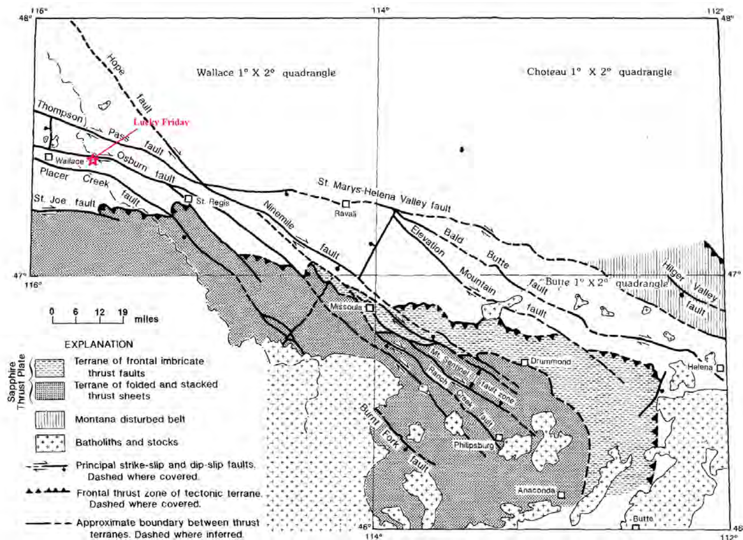
Figure 6-2: Lewis and Clark Line
