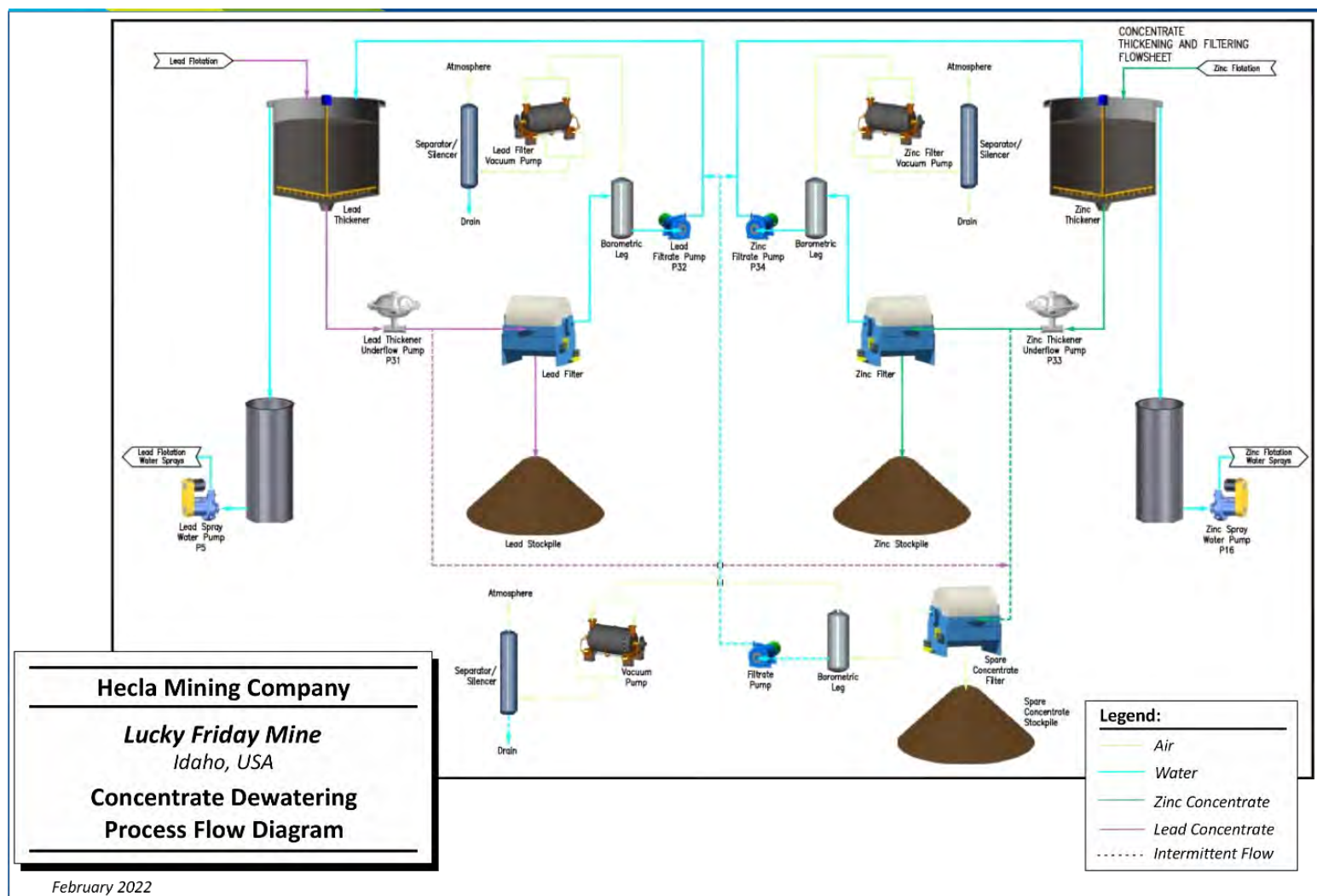
Figure 14-5: Concentrate Dewatering Process Flow Diagram
