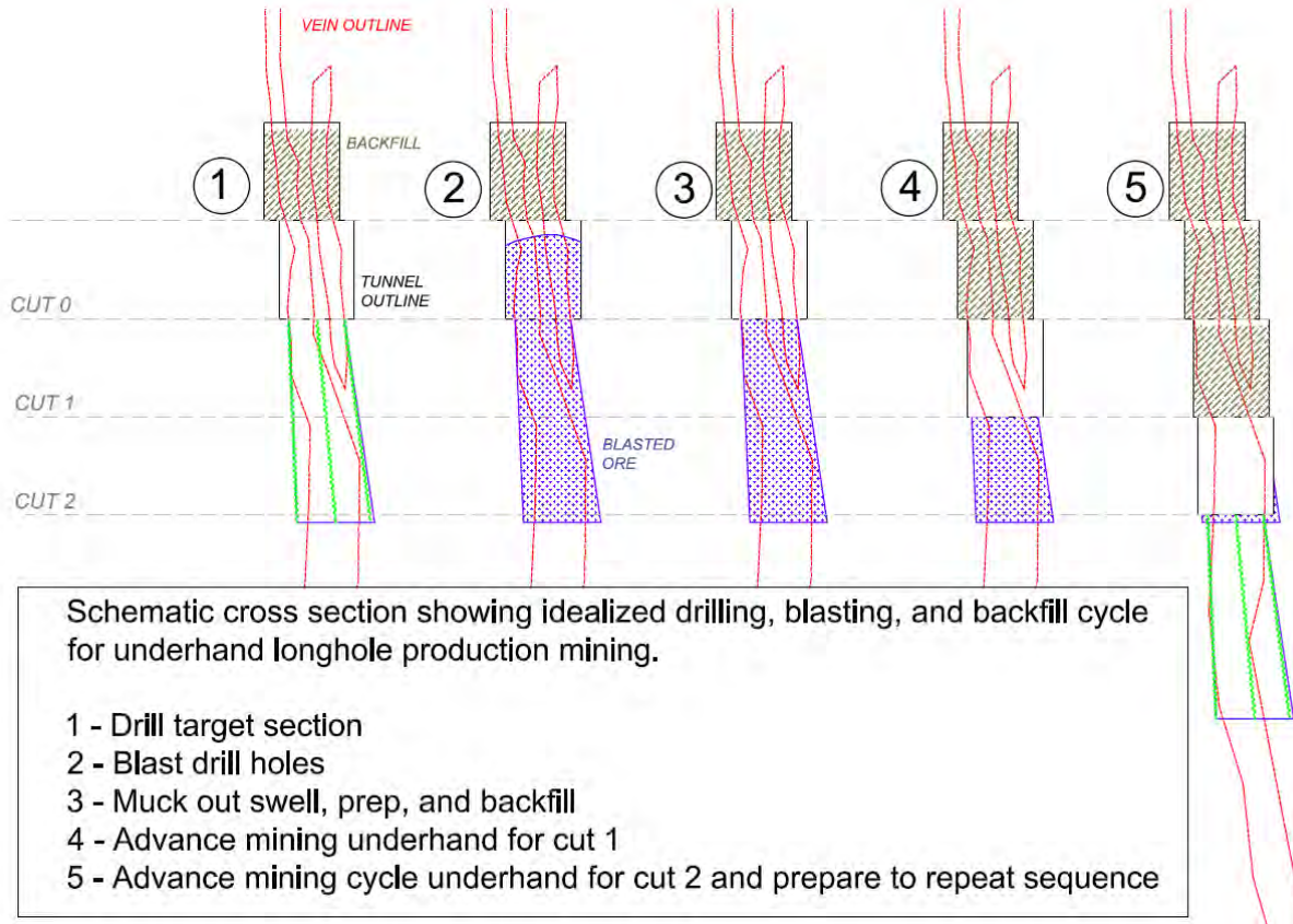
Figure 13-3: Underhand Closed Bench Mining Method Schematic
