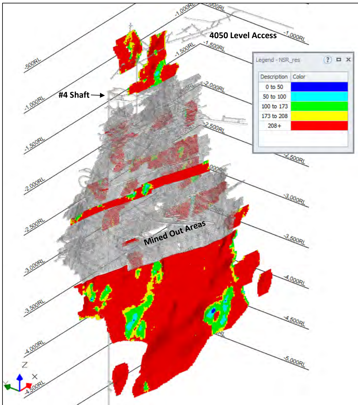
Figure 13-10: Longitudinal Section – Oblique View
