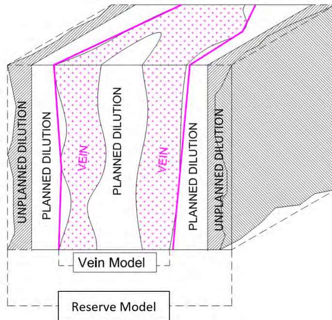
Figure 12-1: Dilution Schematic
