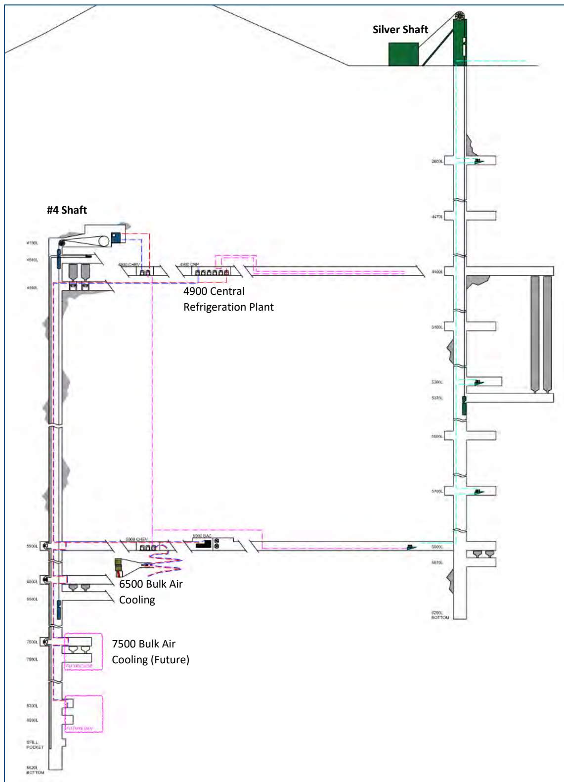
Figure 13-7: Mine Cooling System Schematic
